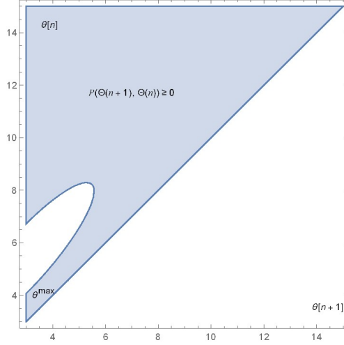
Figure 2: The area where P(\Theta(n+1), \Theta(n)) \geq 0
