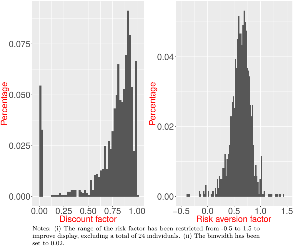
Figure 3: Histogram of the risk aversion and discount factors
